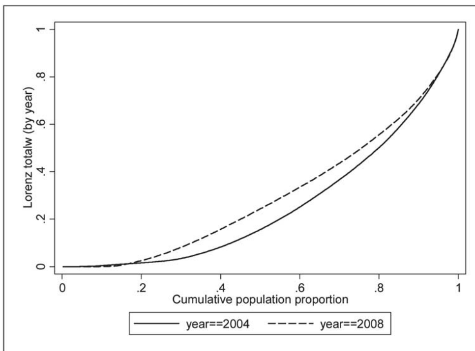
Figure 10: Lorenz Curves for Pre-Tsunami (2004) Total Asset Value and Current (2008) Total Asset Value
