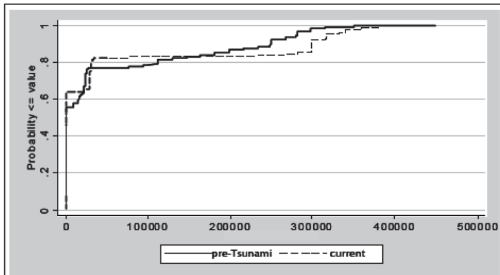
Figure 4: Cumulative Distribution Curves for Current and Pre-Tsunami Boat Values 33
