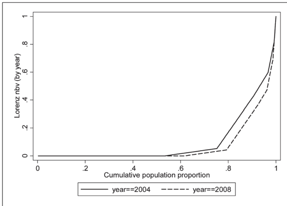
Figure 9: Lorenz Curves for Pre-Tsunami 36 (bv[2004]) and Current Boat Values (bv[2008])
