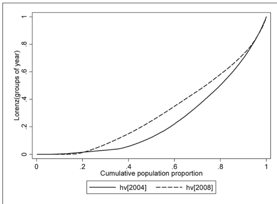
Figure 6: Lorenz Curves for Pre-Tsunami (hv[2004]) and Current House Values (hv[2008])
