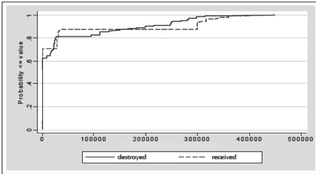
Figure 3: Cumulative Distribution Curves for Value of Destroyed Boats and Boat Aid Received
