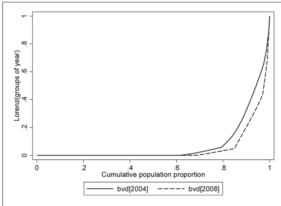
Figure 8: Lorenz Curves for Pre-Tsunami (bv[2004]) and Current Boat Values (bv[2008])
