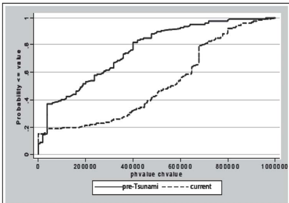
Figure 2: Cumulative Distribution Curves for Pre-Tsunami 32 and Current House Values
