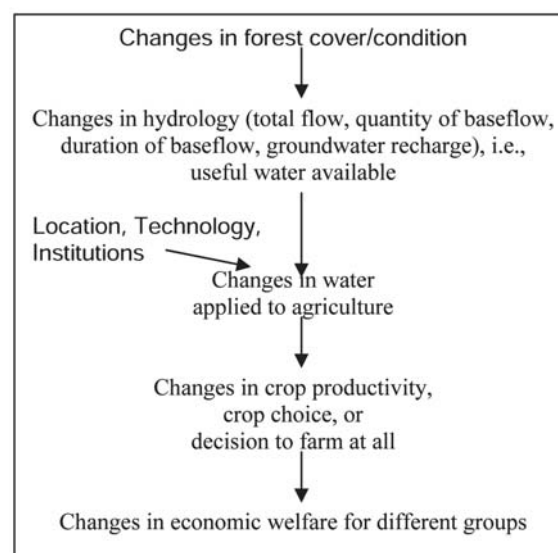
Conceptual Framework
