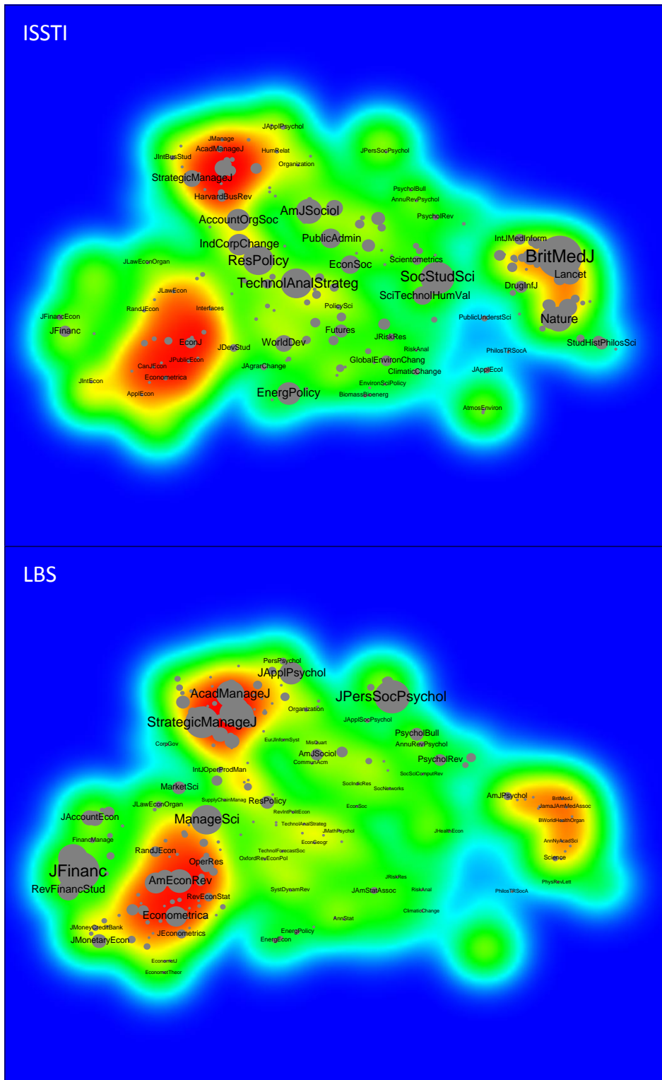
Figure 5. Overlay of the references of ISSTI (Edinburgh) and LBS (London) publications in a local journal map. The map illustrates the similarity structure of the 391 most important journals for all six IS and BMS units analysed. Red areas correspond to a high density of journals, indicating areas of mono-disciplinary activity. Green areas show low density. Node size indicates the proportion of a unit's references in a given journal. Journals located in between red areas, i.e. between disciplinary cores, are interpreted as interdisciplinary. (This figure needs to be viewed in colour).
