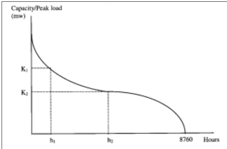
Fig. 1: Load duration curve
