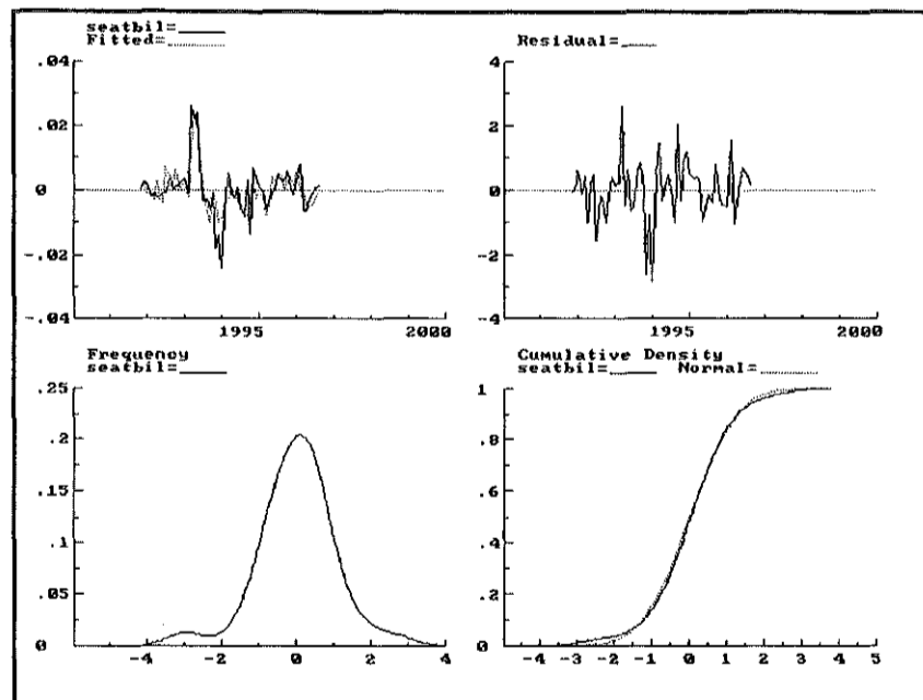
Figure 7: Fitted treasury bill rate results
