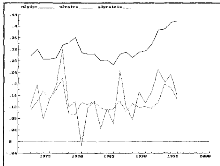
Figure 1: M2/GDP ratio
