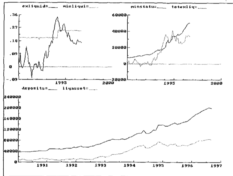
Figure 3: Liquid assets for commercial banks
