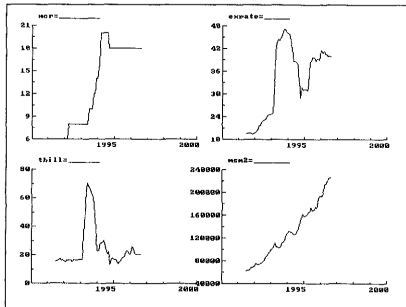
Figure 6a: Impact variables
