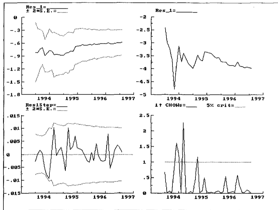
Figure 6a: Impact variables
