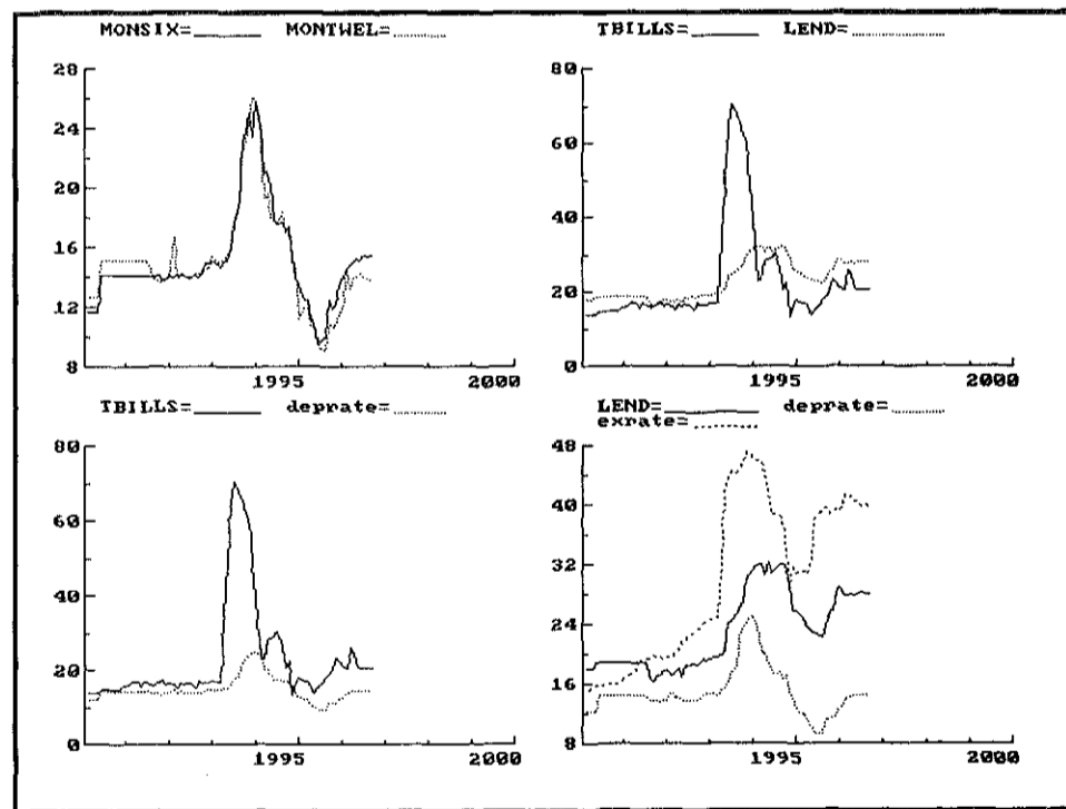
Figure 2: Interest rate spreads
