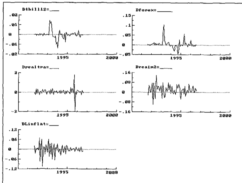
Figure 4: Unit root tests
