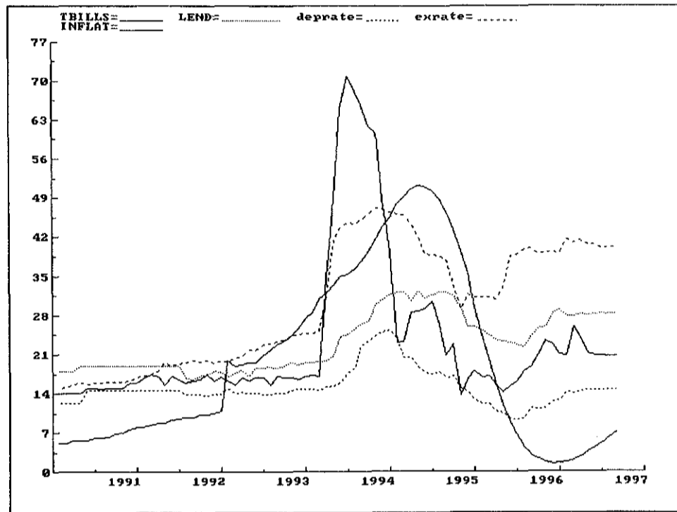
Figure 7: Fitted treasury bill rate results
